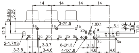
BOTTOM VIEW
