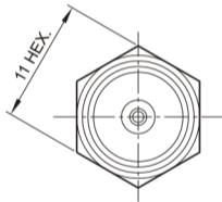
F MALE PLUG
