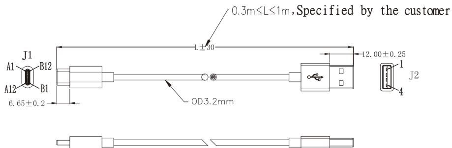
Connection table
